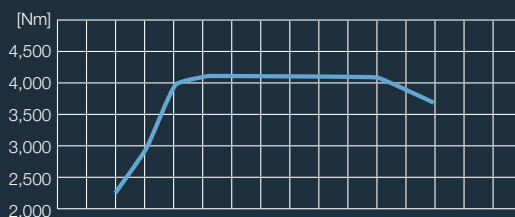
Torque
